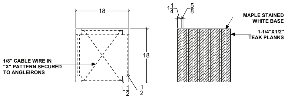
1 COUNTER STOOL BASE DETAILS
