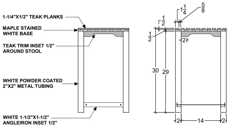
3 COUNTER STOOL SIDE VIEW
