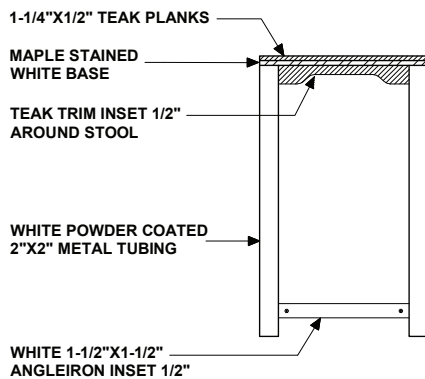
3 COUNTER STOOL SIDE VIEW
